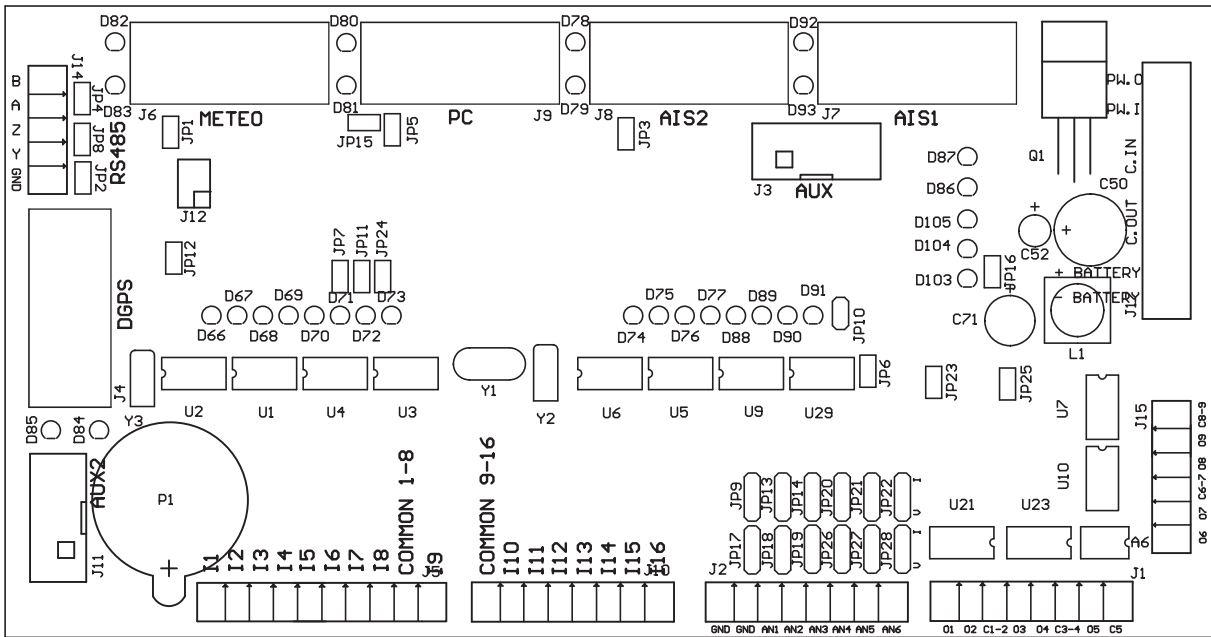
Drawing of a MMB 02 Daughter Board. Dimensions: 191 x 100 mm.
